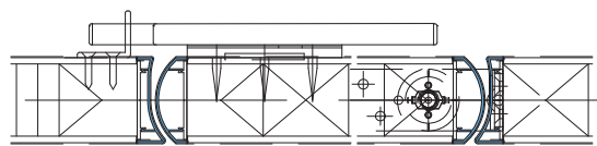
FS:FLUSH SURFACE(同面)
